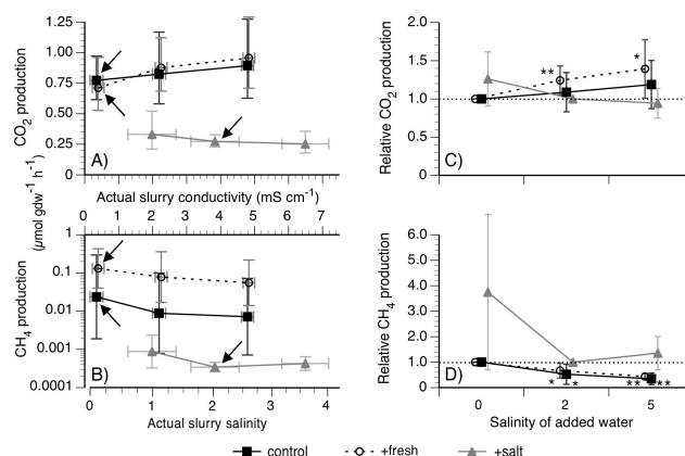
Fig. 2. Short-term effects of elevated salinity on rates of \text{CO}_2 and \text{CH}_4 production. (A, B) Absolute rates of \text{CO}_2 and \text{CH}_4 production as a function of the salinity of the soil slurry. (C, D) Rates of \text{CO}_2 and \text{CH}_4 production relative to gas production at field salinities (salinity = 0 for control and +fresh soils, 2 for +salt soils). Due to porewater already present in the soil, the final salinity of the slurries was somewhat different from that of the added water (see the x axis on panels (A) and (B) for actual slurry salinities). On panels (A) and (B), the data points highlighted with arrows are the same data shown for the 3–8 cm depth interval on Fig. 1 (i.e., rates at field salinities). On panels (C) and (D), asterisks indicate that the relative \text{CO}_2 or \text{CH}_4 production was significantly different than 1.0 (*: p \leq 0.10 ; **: p \leq 0.05 ). Values are means \pm standard deviation, n = 5 plots per data point.
