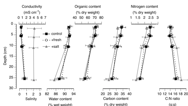
Fig. 4. Soil properties. Values for the control treatment are plotted at the midpoint of each depth interval, with depths for the +fresh and +salt treatments jiggered by \pm 0.5 cm to reduce overlap of symbols and error bars. Values are means \pm standard deviation, n = 5 plots per data point.
