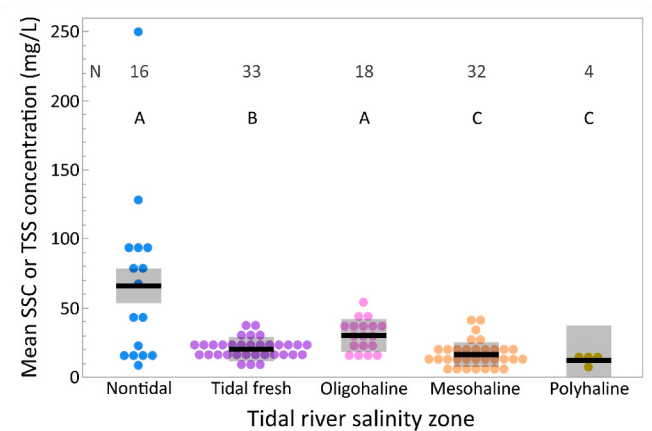
Fig. 3. Monitoring stations’ long-term average suspended sediment concentrations (TSS = total suspended solids; SSC = suspended sediment concentration) measured at nearby nontidal (SSC) and tidal freshwater, oligohaline, mesohaline, and polyhaline stations (TSS) along tidal rivers of the Chesapeake Bay. Sample size (number of stations) is shown at the top of the plot. Different letters indicate significant differences among salinity zones. Mean and 95% confidence interval shown as black lines and gray boxes, respectively.
