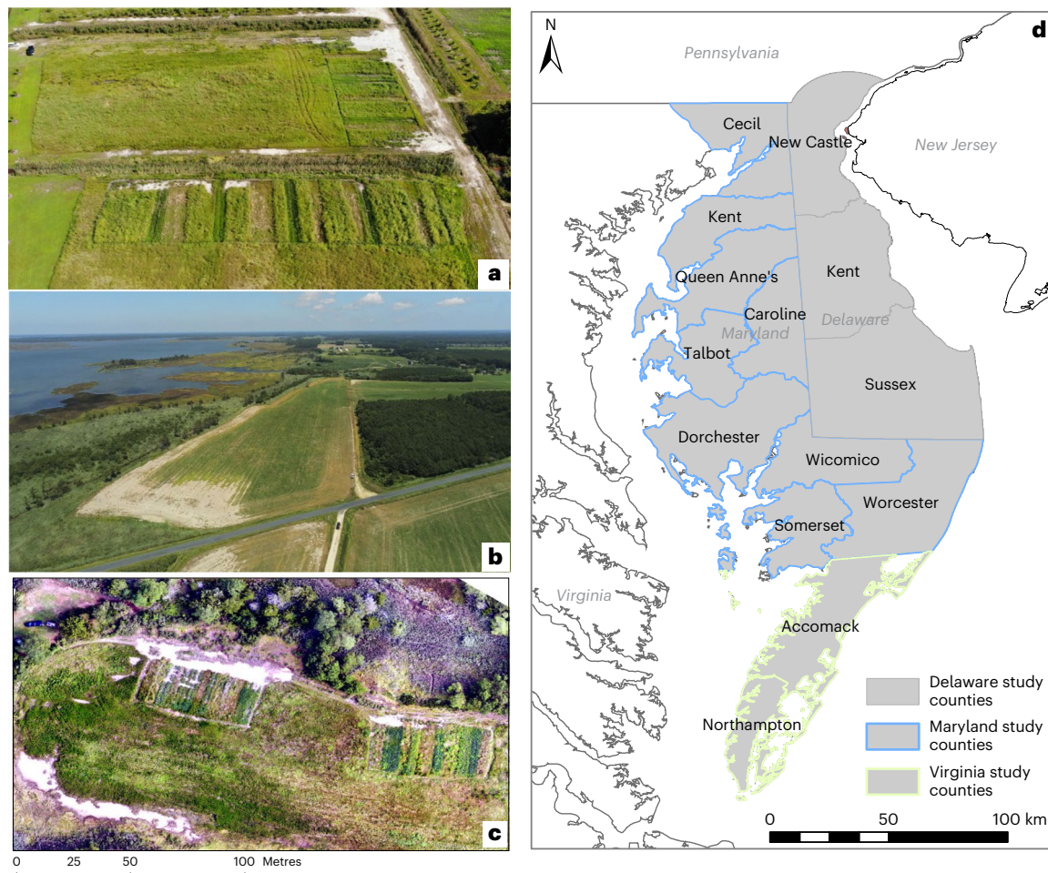
Fig. 1 | Where crops do not grow. a , Visible salt patches at the farm fringes. b , Many Delmarva farmlands are close to brackish or saline water. c , A drone image from a farm in Somerset County, Maryland (2019). d , Study area showing 14 coastal Delmarva counties in Delaware, Maryland and Virginia.
