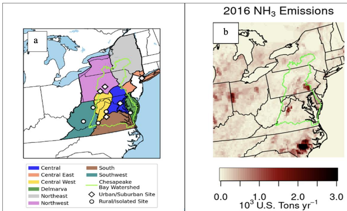
Figure 5. (a) Computational domain and source-apportionment regions used in the CMAQ v5.3.2 Integrated Source Apportionment Method (ISAM) analysis for the northeastern United States. Named source regions encompass the six Chesapeake Bay watershed states (Maryland, Virginia, West Virginia, Delaware, Pennsylvania, and New York). The area within the modeling domain but outside these states is referred to as the region outside the watershed states. National Atmospheric Deposition Program (NADP) National Trends Network (NTN) monitoring locations are shown as diamonds (urban or suburban sites) and circles (rural or isolated sites). Figure adapted from Benish et al. (2022); (b) Annual \text{NH}_3 emissions from the U.S. Environmental Protection Agency (EPA) 2017 National Emissions Inventory (NEI) with the corrected Maryland animal emissions.
