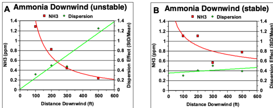
Figure 9. Downwind \text{NH}_3 concentrations (broiler production). Daily average \text{NH}_3 concentrations under unstable (daytime) conditions (left) and stable (nighttime) conditions (right). Under unstable conditions, \text{NH}_3 concentrations decrease rapidly with downwind distance following a power-function relationship, and the climatic dispersion effect increases sharply. Under stable conditions, \text{NH}_3 concentrations decrease only minimally with distance, and the climatic dispersion effect shows little change. Climatic dispersion effect is defined as the variance of the daily \text{NH}_3 concentration divided by the daily mean concentration. Figure adapted from materials presented in the STAC workshop (STAC 2022; https://www.chesapeake.org/stac/wp-content/uploads/2022/05/SPAC-Presentation-2022-print.pdf ).
