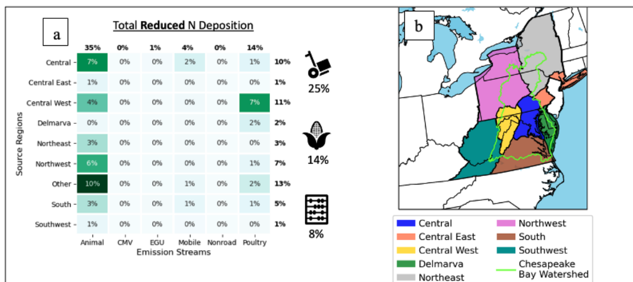
Figure 7. (a) Relative contributions of modeled emission streams and source regions to total reduced nitrogen deposition in the Chesapeake Bay watershed. Values shown in the heat map represent the percent contribution of each source region–emission stream combination to total reduced N deposition, with row and column totals shown at right and top, respectively. Agricultural and poultry-related sources comprise the largest shares of reduced N deposition in this analysis. Figure informed by regional nitrogen deposition analyses in Benish et al. (2022); adapted for Chesapeake Bay source-apportionment results presented here, This analysis was completed before the 2017 NEI emissions error was identified. Updated values for the Central West, Central, and Delmarva regions are in Tables 3-6; (b) CMAQ v5.3.2 Integrated Source Apportionment Method (ISAM) modeling domain for the Northeastern United States, showing the 12-km grid and the Chesapeake Bay watershed States (Maryland, Virginia, West Virginia, Delaware, Pennsylvania, and New York). https://acp.copernicus.org/articles/22/12749/2022/acp-22-12749-2022.pdf
