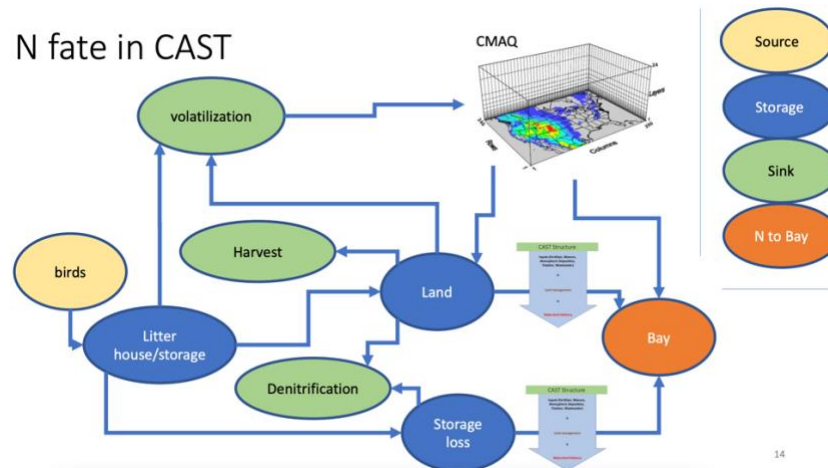
Figure 3. Conceptual diagram showing how poultry-derived nitrogen moves through manure, volatilization, deposition, land application, and delivery to the Bay. Source: Gary Shenk, Poultry Sources in Chesapeake Bay Program Nitrogen Modeling (STAC presentation).
