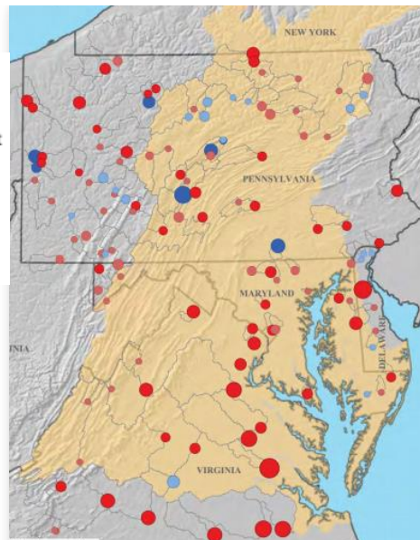
Figure 1. Locations of stream-water temperature measurement stations and results of trend analyses at those stations, Chesapeake Bay region, 1960–2014.
