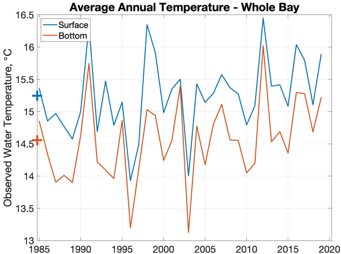
Figure V-3. Observed annual averaged surface and bottom water temperatures across Chesapeake Bay from 1985 through 2020. Source: Hinson et al. 2021.
