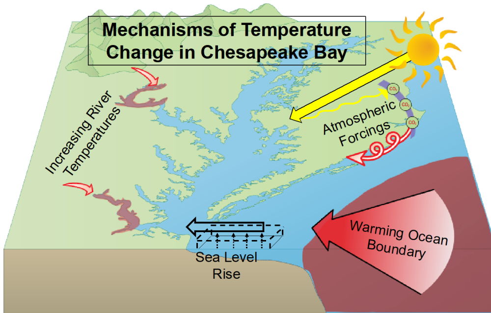
Figure V-6. Illustration of the four major mechanisms driving changes in water temperature throughout the Chesapeake Bay's mainstem, tidal tributaries and embayments. Source: Hinson et al. 2021
