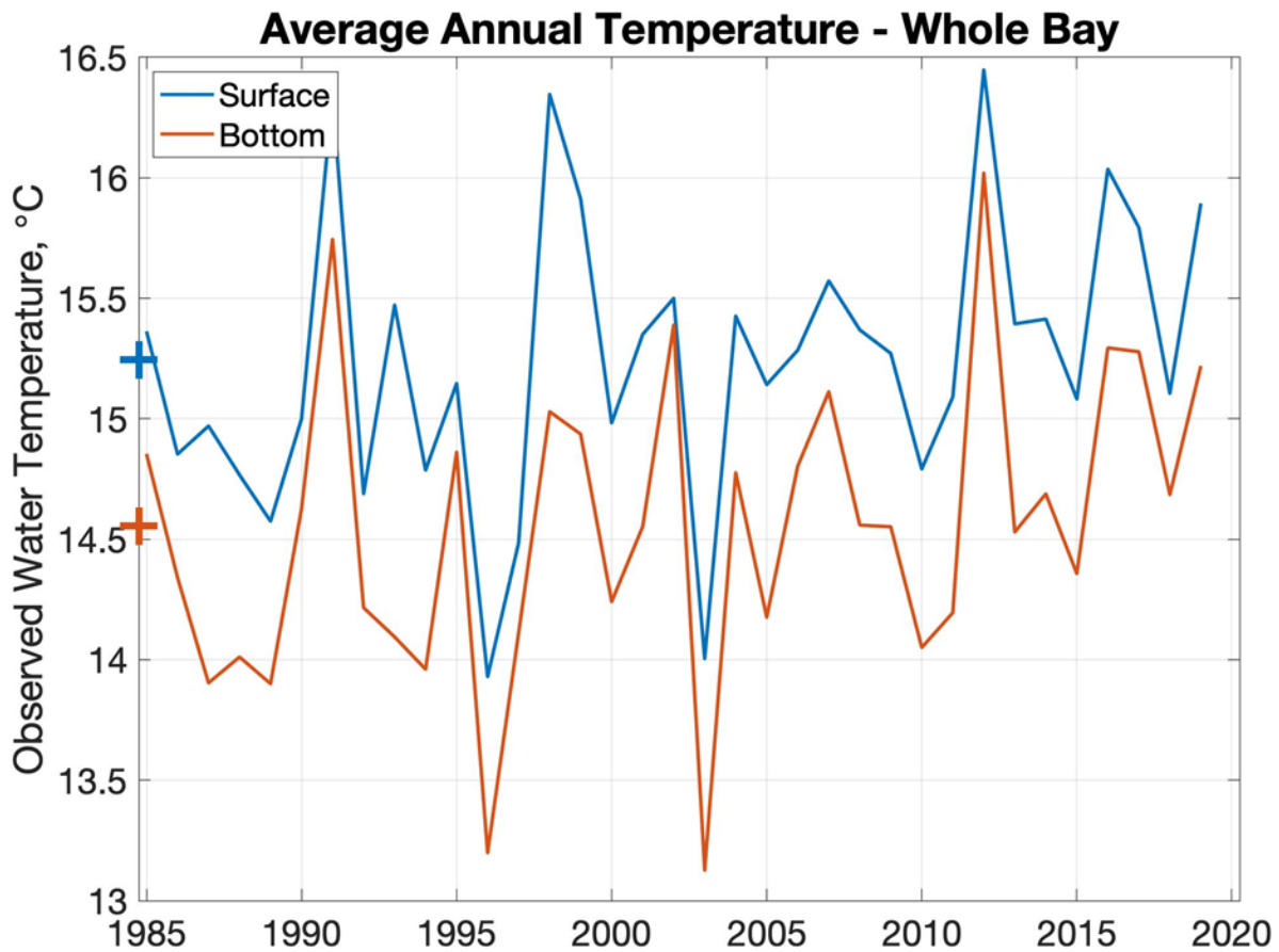
Figure V-1. Observed annual averaged surface and bottom water temperatures across Chesapeake Bay from 1985 through 2020. Source: Hinson et al. 2021.
