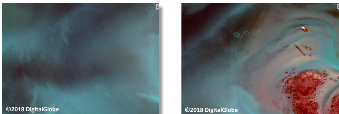
Figure 3. Propeller scars (left) and hydraulic clam dredge scars (right) detected using satellite imagery. (Imagery ©2018 DigitalGlobe)
