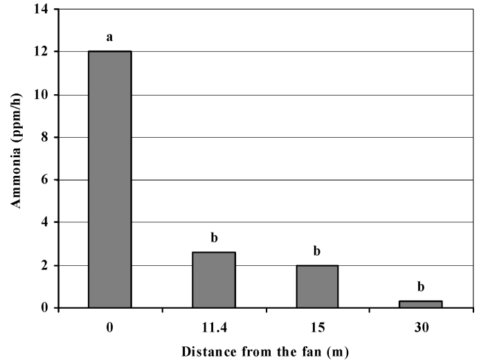
Fig. 2. Aerial ammonia ( \text{NH}_3 ) concentrations measured at 0, 11.4, 15, and 30 m downwind of the fans from all five commercial poultry farms (a, b denote significant differences [ P \leq 0.05 ]; standard error of the means (SEM) = 0.78).
