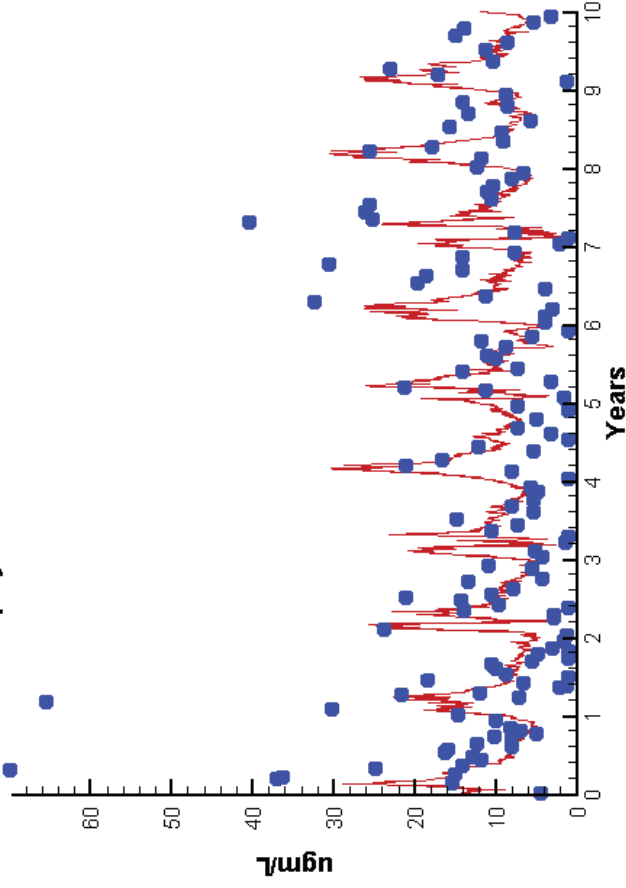
Run184 1991-2000 Chlorophyll RET3.2 Surface
