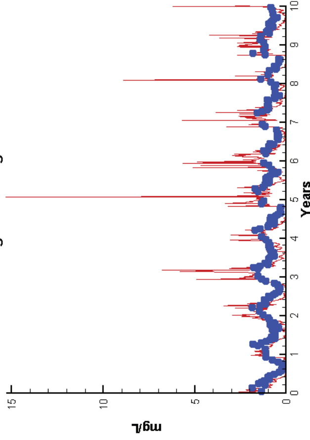
Run184 1991-2000 Dissolved Inorganic Nitrogen CB2.2 Surface
