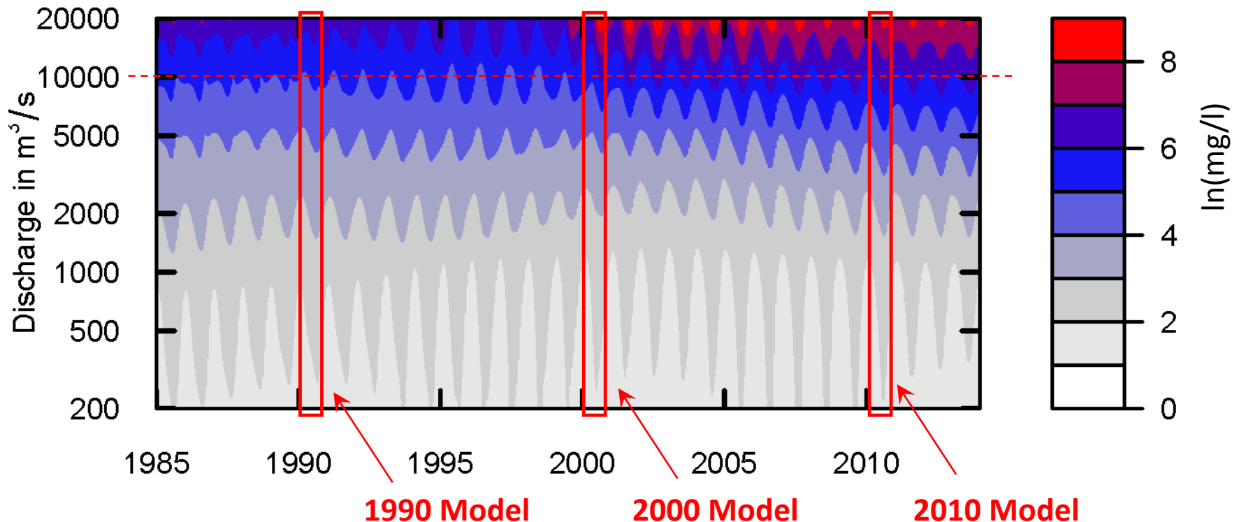
Estimated log of Concentration Surface in Color
