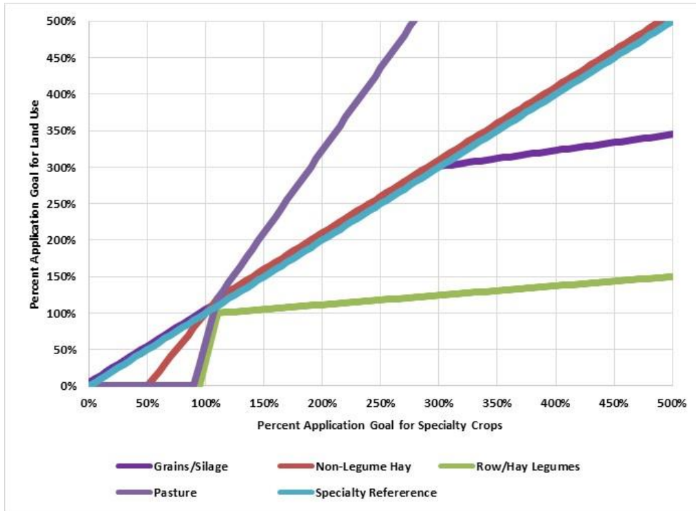
Figure 3-5: Inorganic Nitrogen Application Curves by Crop Group
