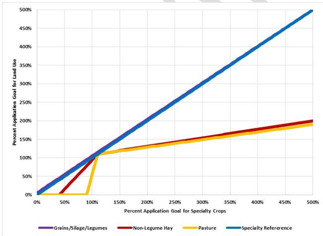
Figure 3-6: Inorganic Phosphorus Application Curves by Crop Group
